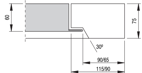
DETALLE A DETAIL A
