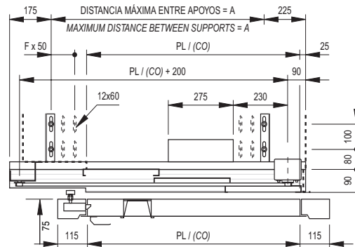
SEMIAUTOMÁTICA CON LADO CONTRARIO / HINGED DOOR WITH OPPOSITE SENSE OF C
