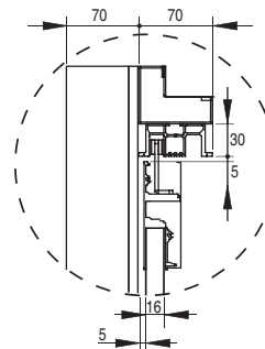
Detalle 1 Detail 1
