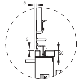
Detalle 2 Detail 2
